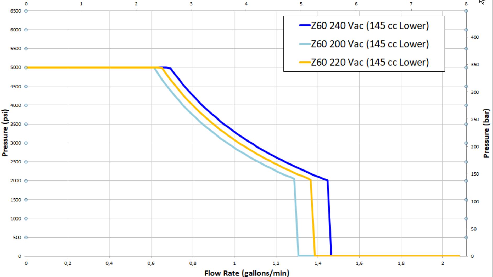
Pressure-Flow Curves
